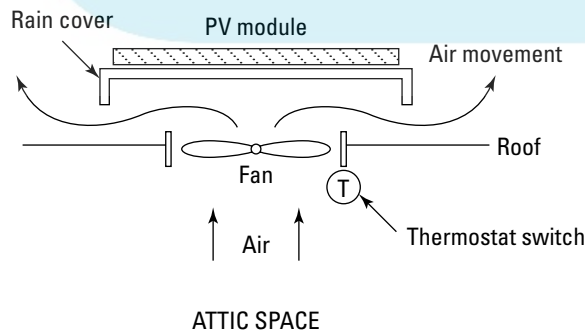
Figure 13-9: One-piece attic vent fan units are very easy to install.
